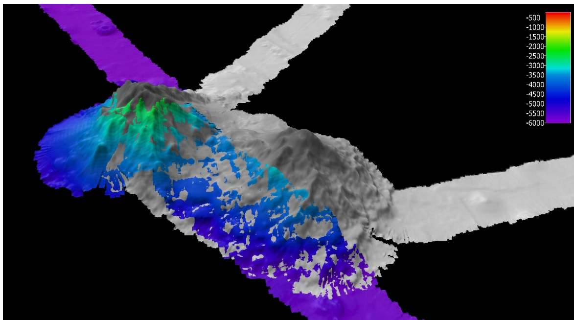
Figure 22. Rainbow bathymetry from EX-17-08 and bathymetry from EX-17-07 in grey over Mussorgsky Seamount. When possible, mapping operations on EX-17-08 leveraged existing coverage from EX-17-07.
