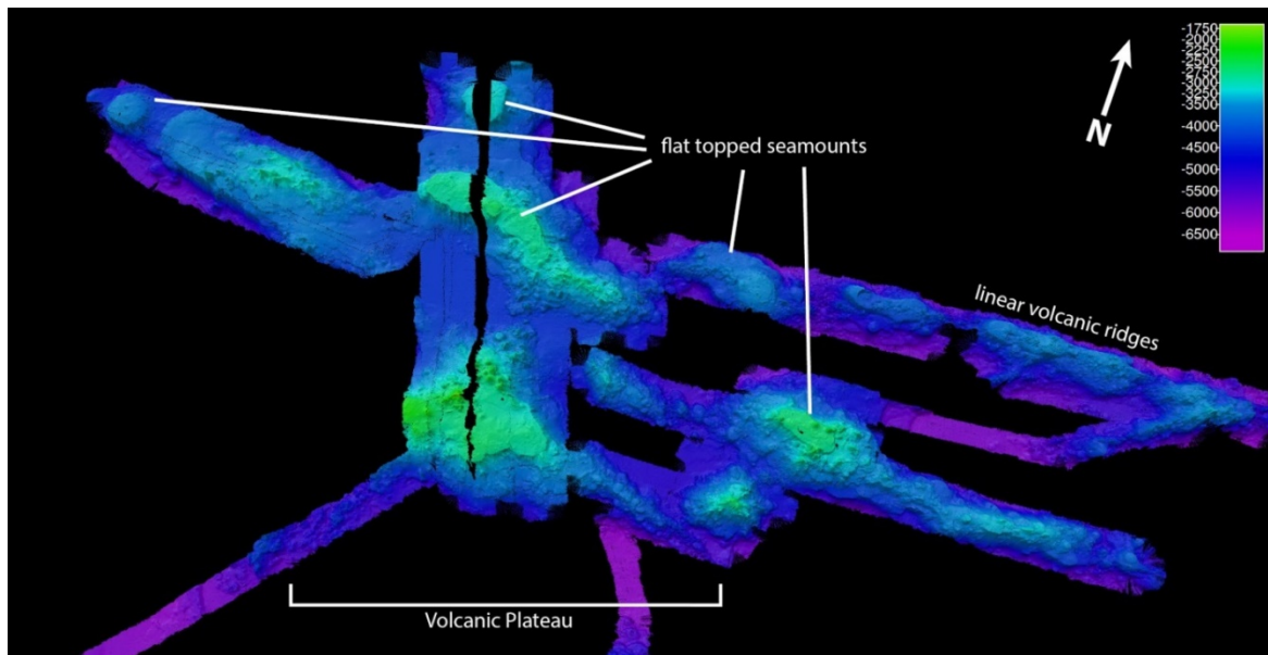
Figure 3. New mapping data along the northern extent of the expedition operating area revealed an elevated volcanic plateau with several guyots and linear volcanic ridges. Courtesy of Eric Mittelstaedt.
