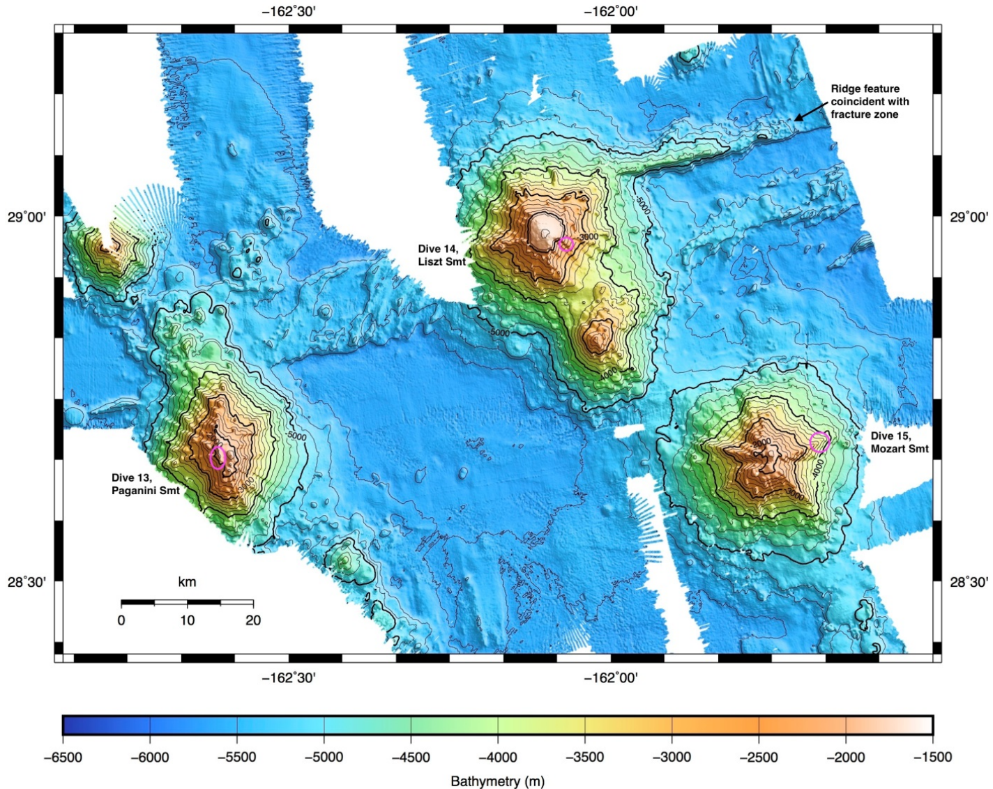
Figure 4. Multibeam bathymetric synthesis for the three seamounts discussed within this section: Paganini, Liszt, and Mozart Seamounts (Dives 13-15, magenta circles). Grid cell interval at 60 m, 200 m contours, bold every 1,000 m.
