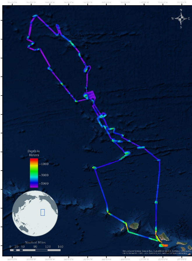
Figure 21. Map showing cruise track and multibeam bathymetry collected during EX-17-08. This cruise began and ended in Honolulu, Hawai‘i.
