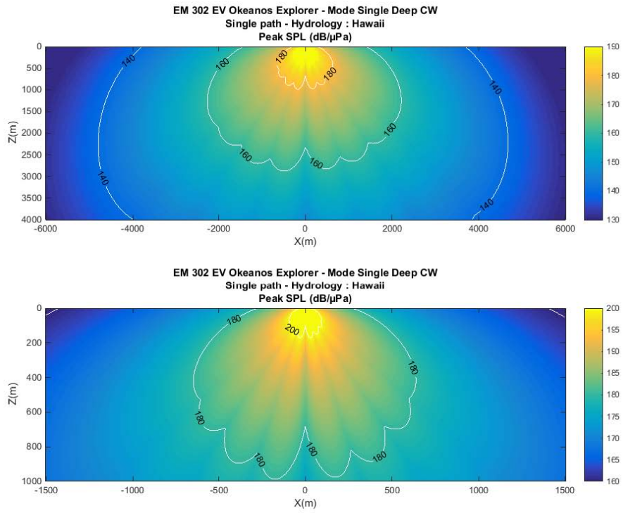
Figure B: Vertical plane view of sound pressure levels in the water column directly below the EM302 sonar transducer.
