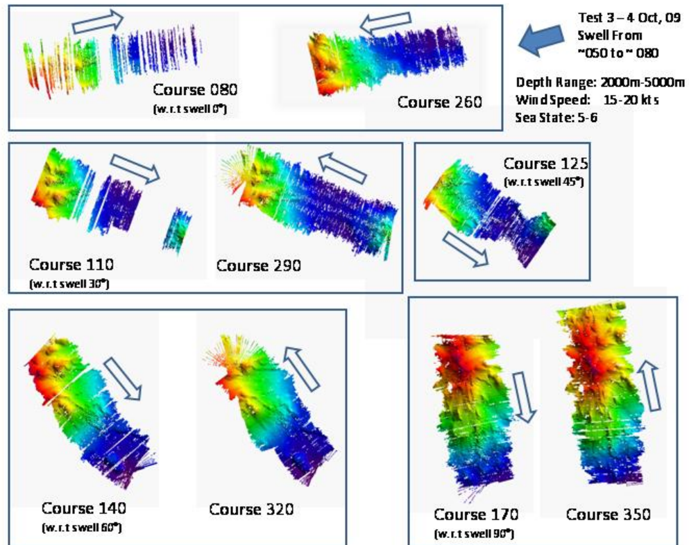
Figure 10: Image showing mapping results with lines run over Wini seamount in different directions
