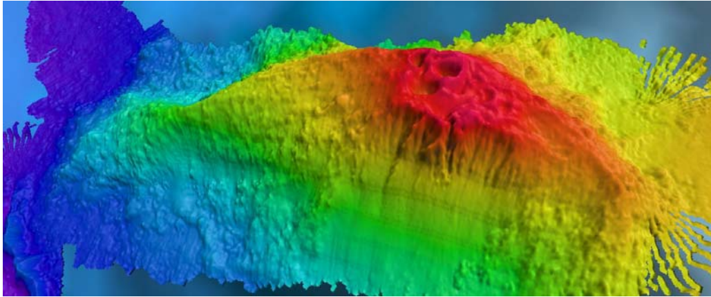
Figure 7: Bathymetric results over Loihi seamount.
