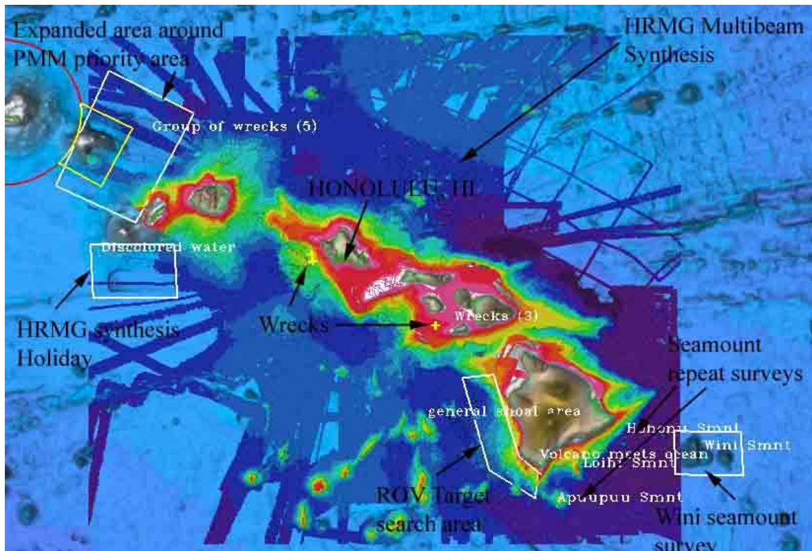
Figure 1: Over view of planned mapping areas during EX0909_Leg 3 cruise (shown as white boxes).
