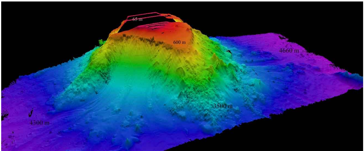
Figure 9: Preliminary results of the EM 302 bathymetric data over the PMNM priority area.
