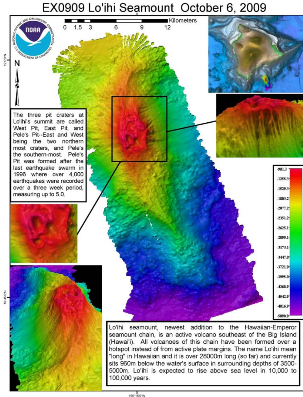
Figure B1: Map sheet showing Loihi seamount. Data credit: NOAA Okeanos Explorer. Map sheet created by Elaine Stuart.
