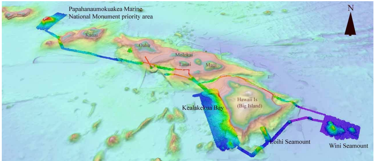
Figure 2: Over view of the EX0909 Leg mapping areas overlaid with bathymetry from ETOPO 1 [8].
